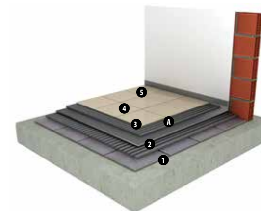
1- floor slab 2- old floor tile 3- fonopac r 4- floor tile 5- bandin A- cement-based adhesive + unilax
